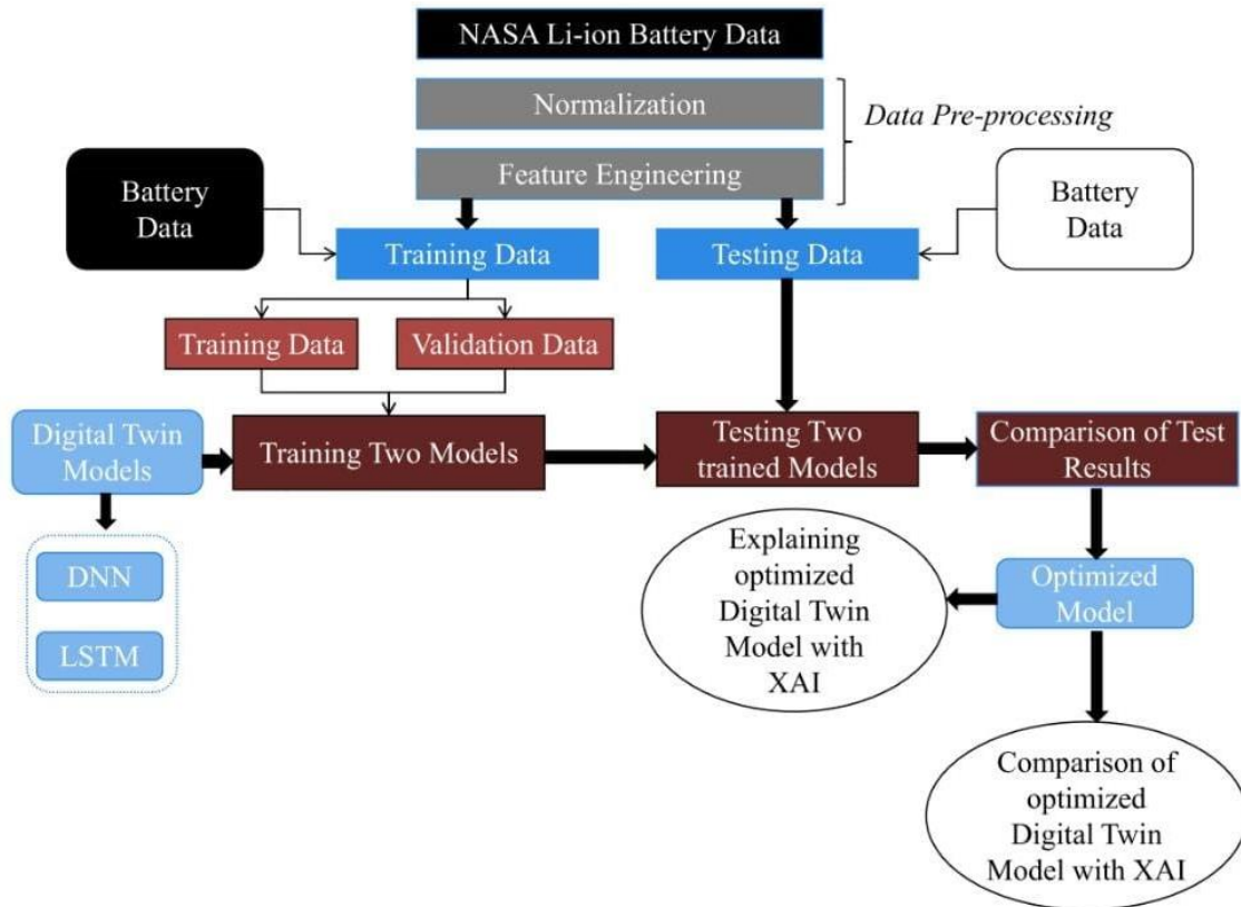
Figure 3.1: Overall design of the study for XAI and digital twin-based state estimation of electric vehicles.
