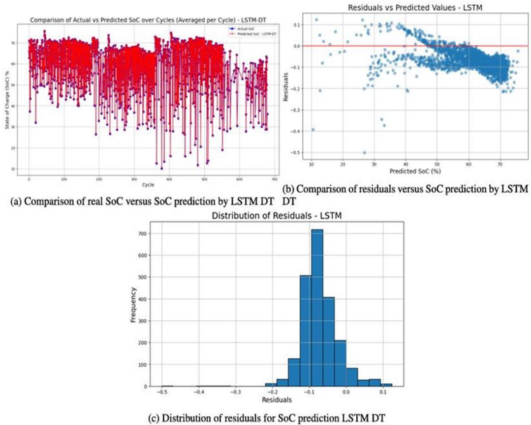
Figure 5.1 : Visualizations of SoC Predictions and Residuals using LSTM DT
