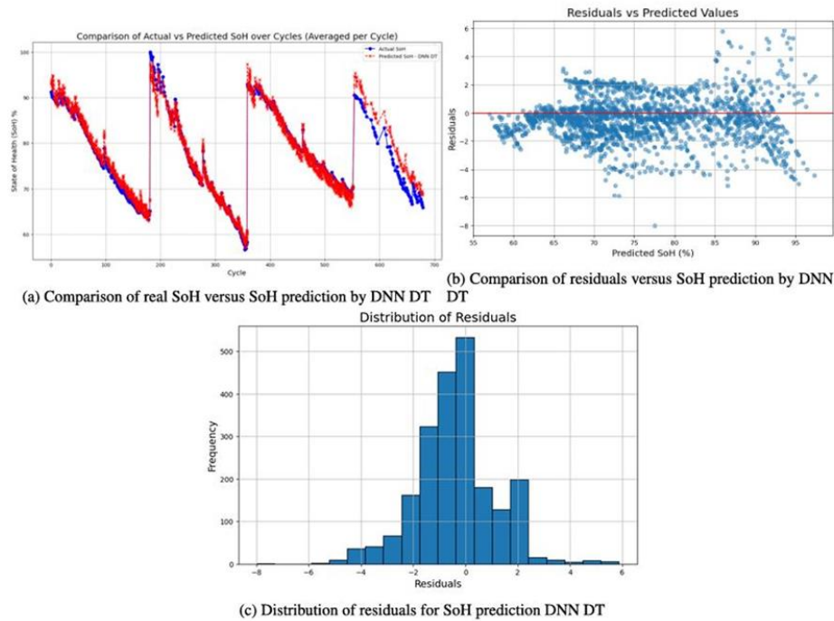
Figure 5.2: Visualizations of SoH Predictions and Residuals using DNN DT
